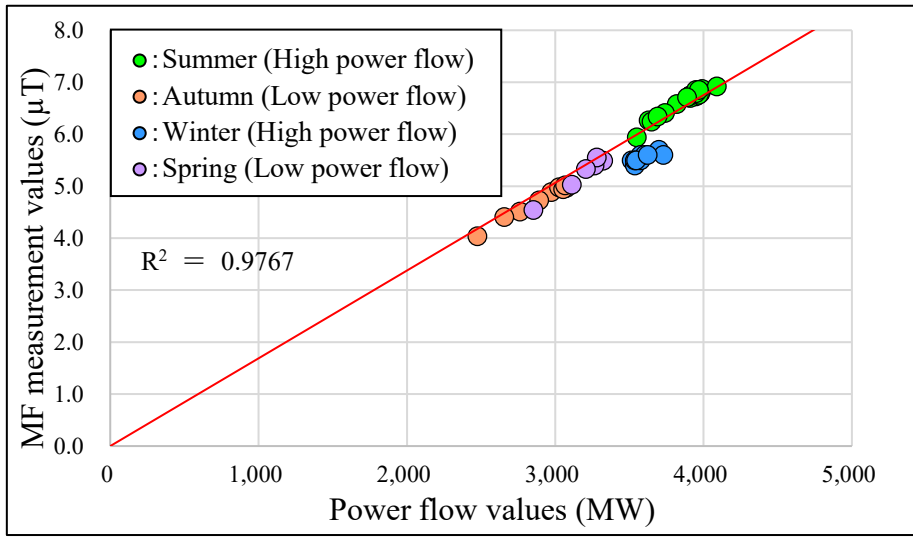
Figure Relationship between power flow values and MF measurement values
